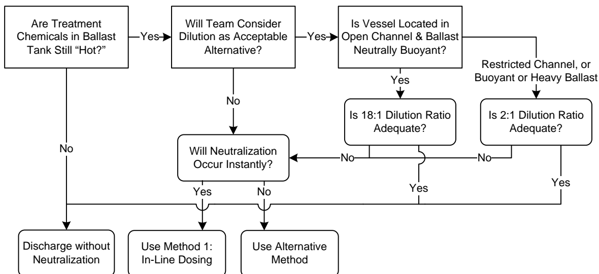
Figure 16 - Neutralization Flow Chart
