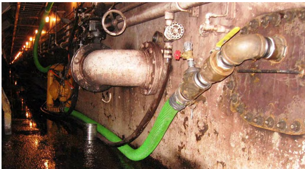
Figure 10 - Chemical Injection Manifold Tee Fitting Shown, Transfer Pump in Background
