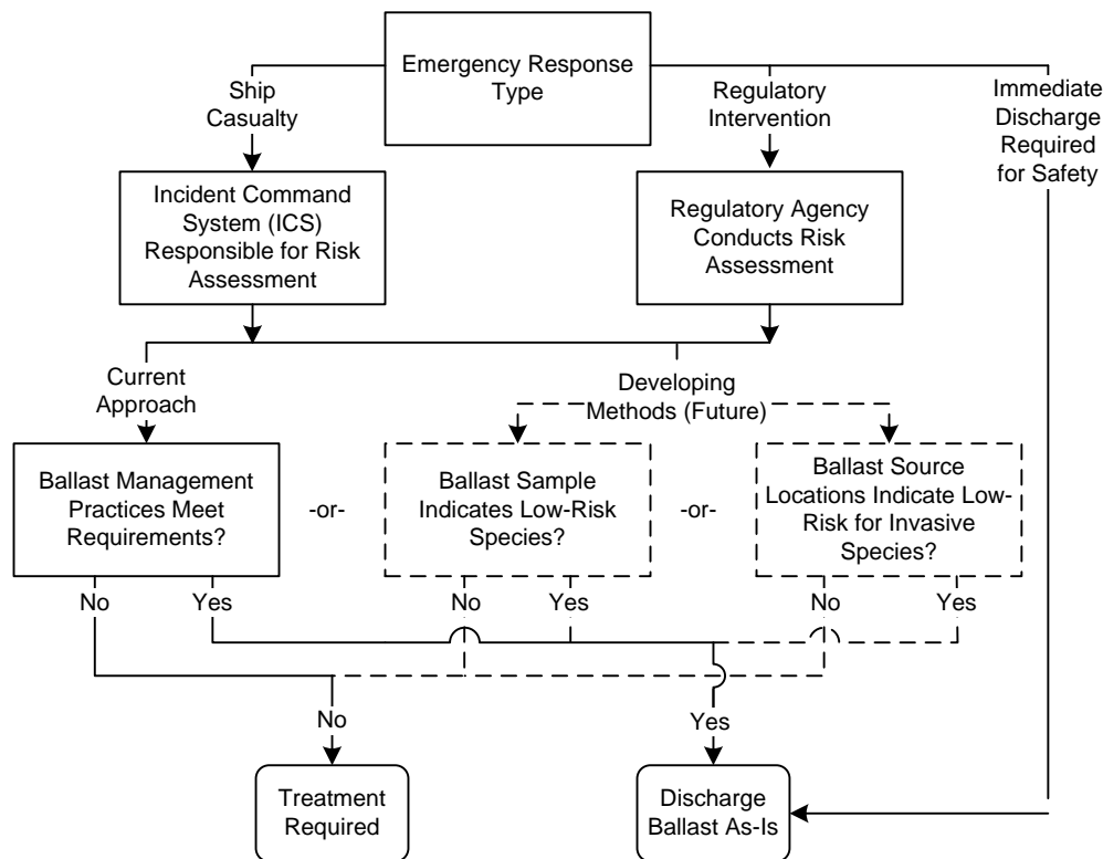
Figure 3 - Risk Assessment Flow Chart
