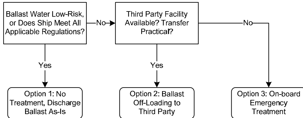
Figure 4 - Response Approach Flow Chart
